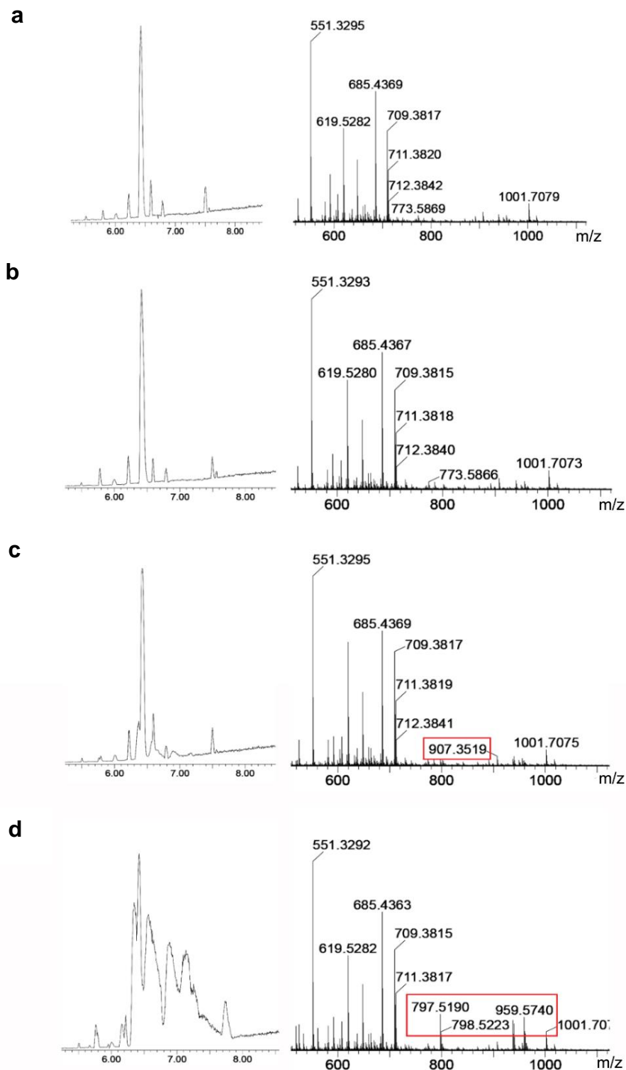
Fig. 3. Total ions chromatogram (left) and mass spectrometry (right) detection of OeB extracts with different ethanol concentrations. The OeB standard product dissolved in: 10% ethanol (a); OeB extracted by 10% ethanol (b); OeB extracted by 30% ethanol (c); and OeB extracted by 60% ethanol (d) (Note: The abscissa is time in total ions chromatogram, and the numbers shown in the mass spectrometry are molecular weights)
