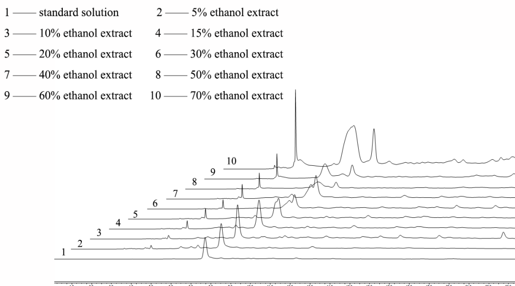
Fig. 2. Extraction effect of OeB with different ethanol concentrations (standard solution dissolved in 10% ethanol)
