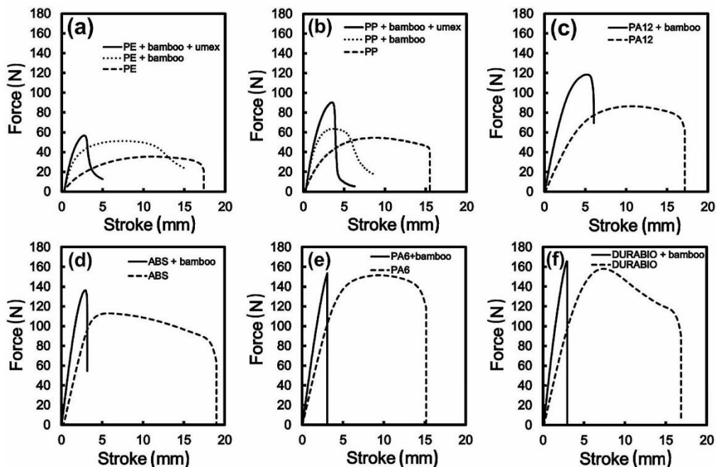
Fig. 8. Flexural Load-Displacement curves of fiber-reinforced composites at 30 wt% fiber and polymer composites: (a) PE, (b) PP, (c) PA12, (d) ABS, (e) PA6 and (f) Durabio
