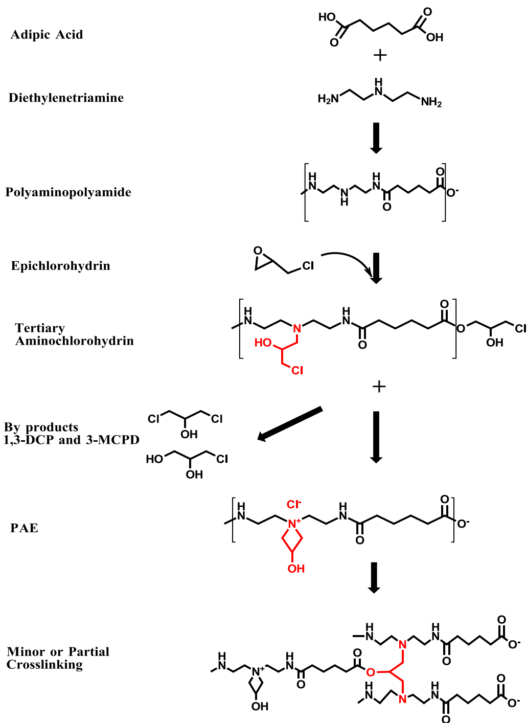
Fig. 1. General steps of PAAE production
