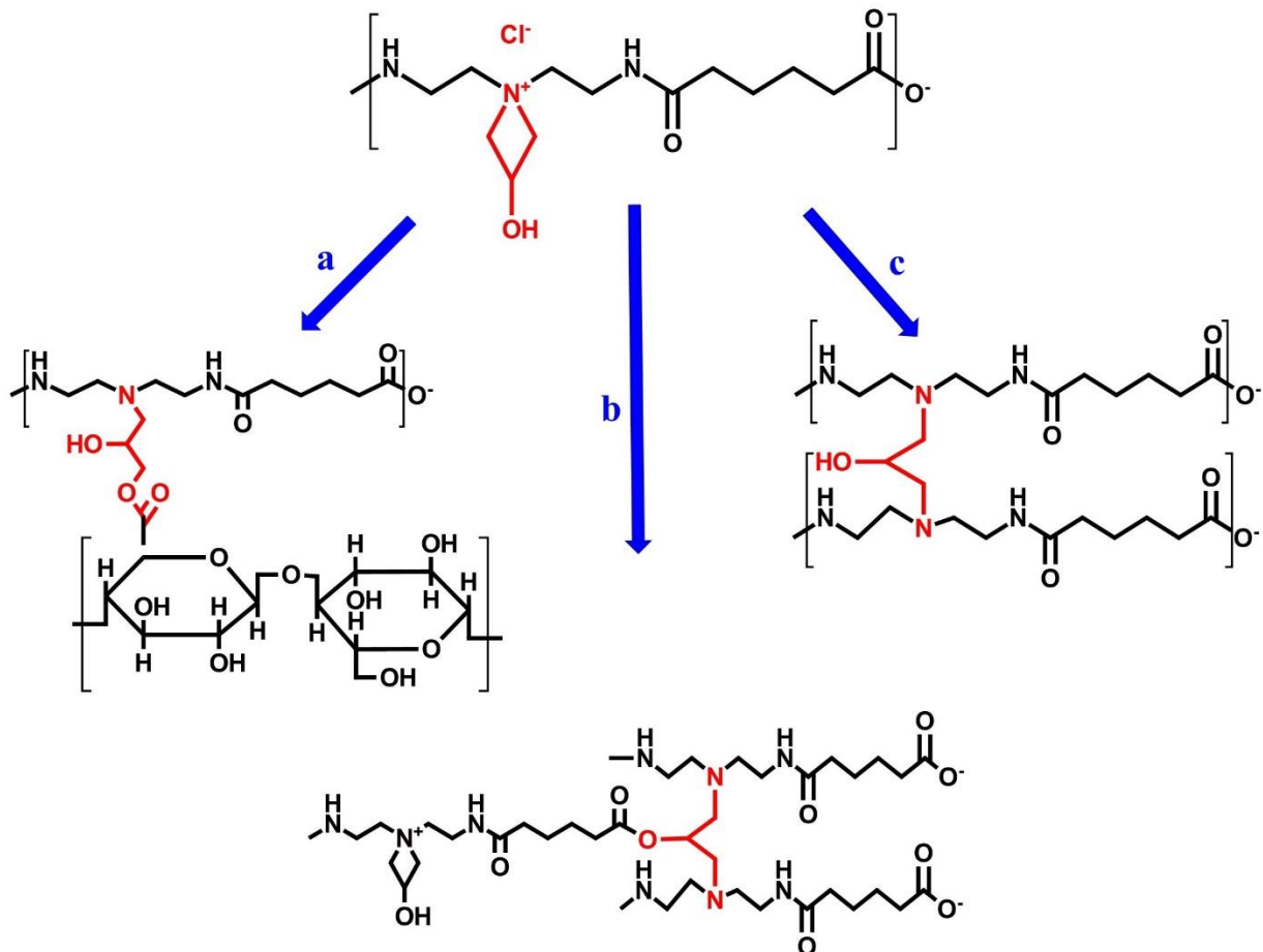
Fig. 2. Structure of PAAE (top), PAAE forming ester bond with cellulose (path a), PAAE main cross linking (path b) and PAAE secondary cross linking (path c)
